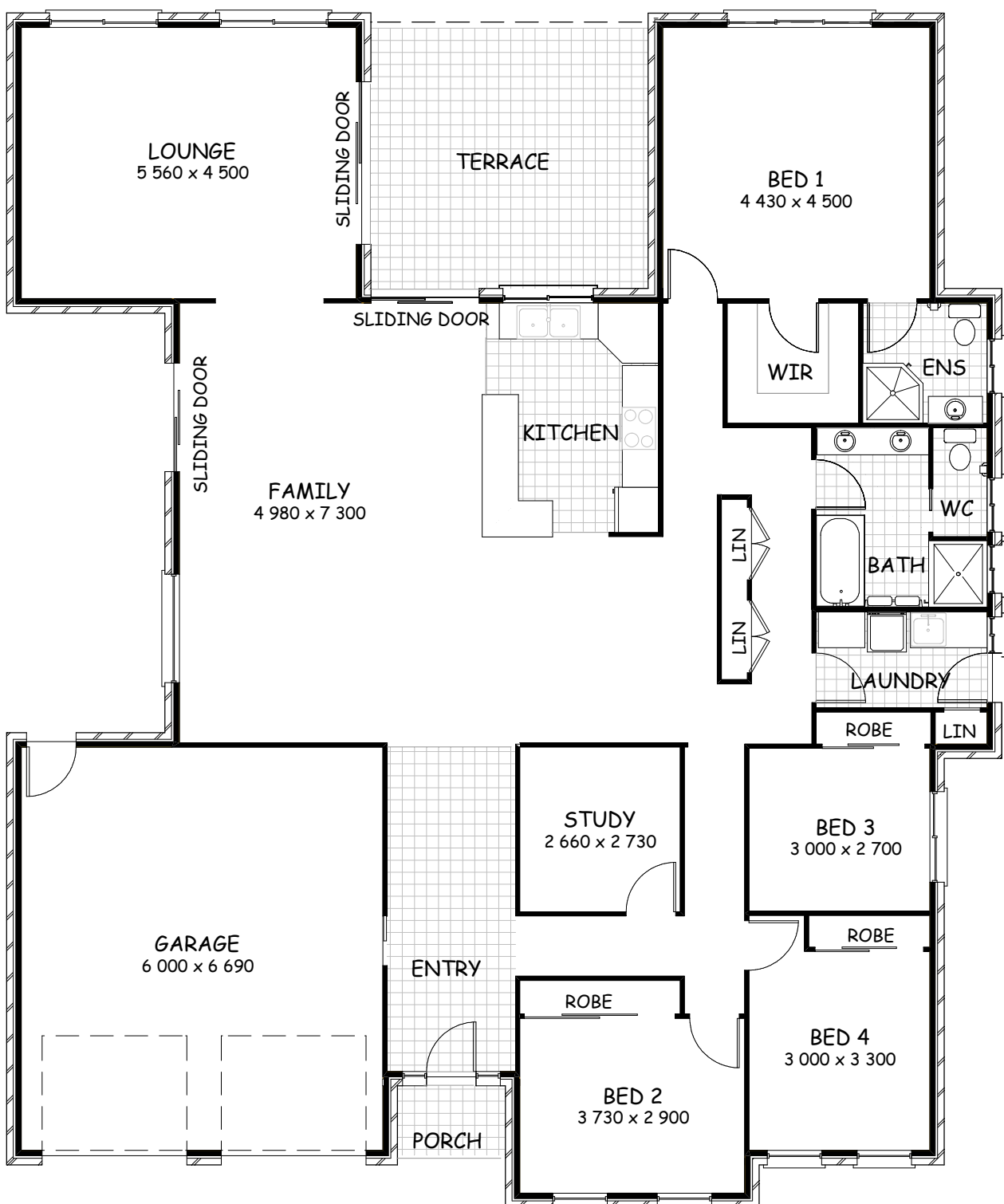
FLOOR PLAN
